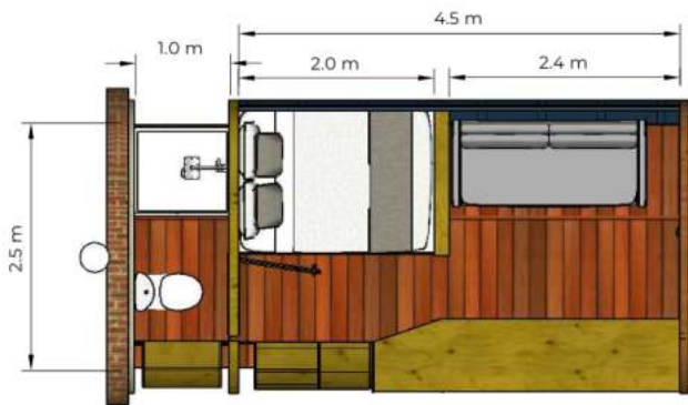
Interior plan
