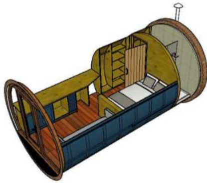
Interior plan
